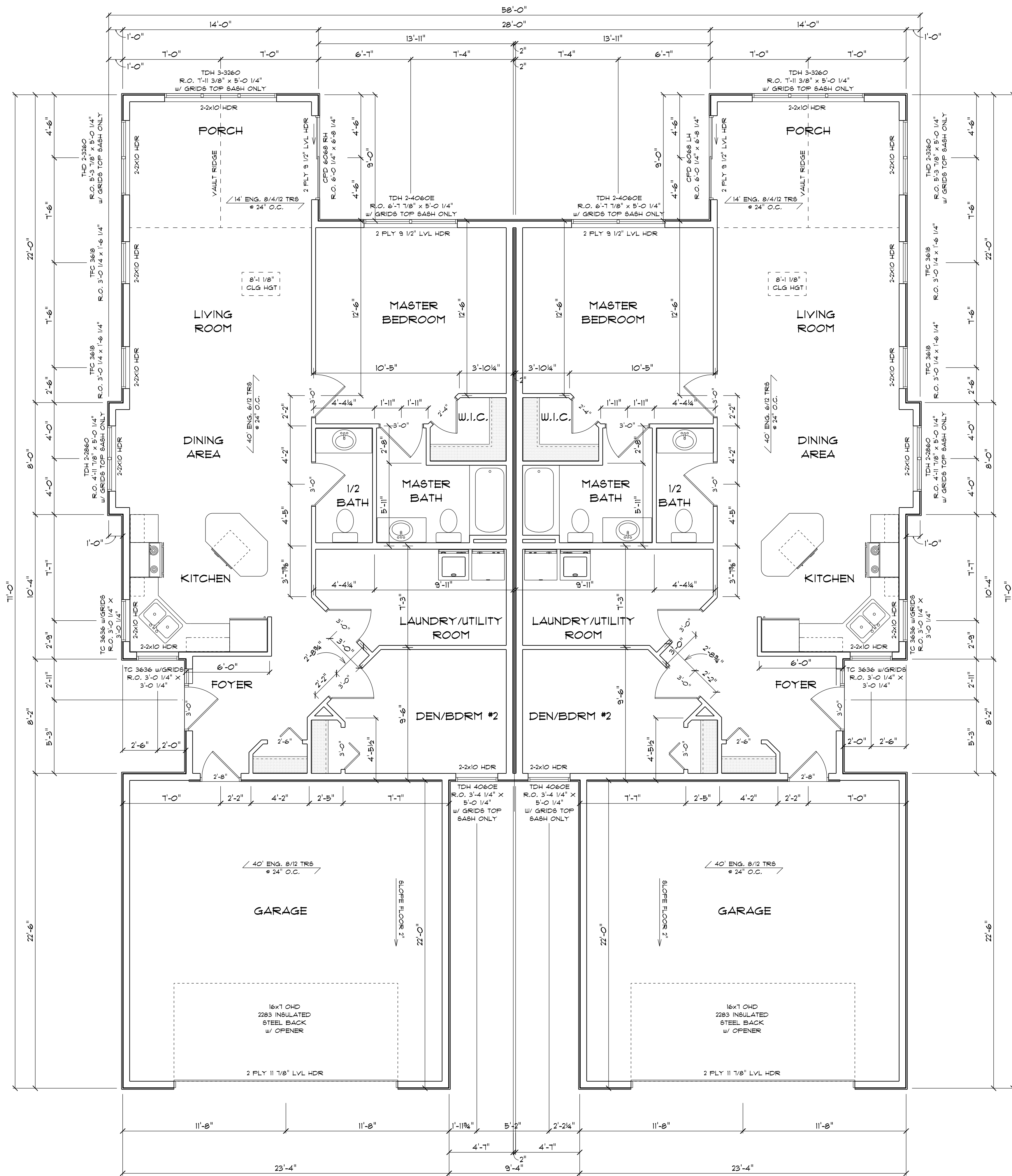
FLOOR PLAN SCALE: 1/4" = 1'-0" 5-31-19
